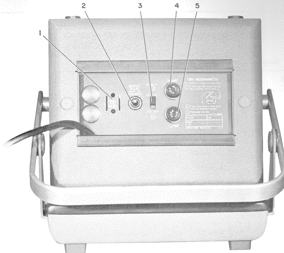
Figure 1-3. Type 1864 rear-panel controls and connectors.
