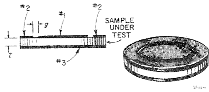
Figure 4-1. Electrode arrangement for resistivity measurements.
