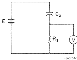
Figure 4-2. Basic megohmmeter circuit.
